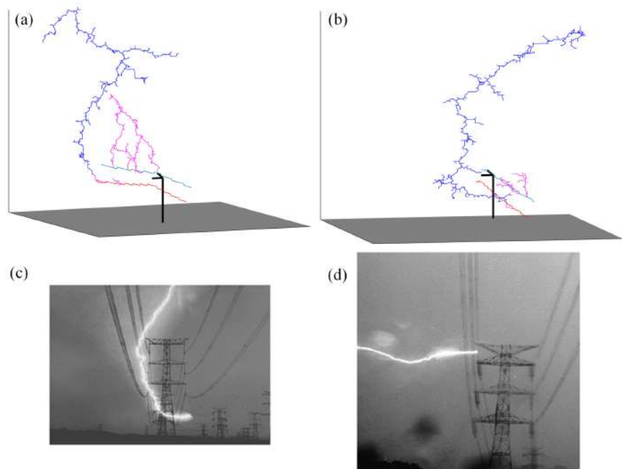
(a), (b) Shielding failure cases based on stochastic model results 1 (c), (d) still photographs of shielding failures to transmission line in Japan 2 .
